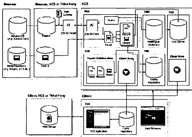
Fig. 2: Architectural overview of the Hypermuseum system.
